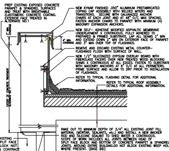
01 PARAPET FLASHING DETAIL SCALE: 1 1/2" = 1' - 0"
