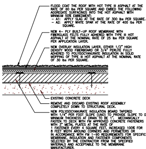
A1/A2 TYPICAL ROOF ASSEMBLY DETAIL "A" SCALE: 1 1/2" = 1' - 0"
