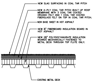
A TYPICAL ROOF ASSEMBLY 'A' SCALE: NTS ROOF AREAS ALL EXCEPT 1, 2, 3, 4
