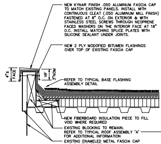
01 TYPICAL FASCIA SCALE: NTS
