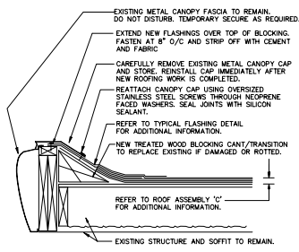
24 ENTRY CANOPY FASCIA DETAIL SCALE: 1 1/2"=1'-0"
