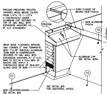
17 CHEEK WALL DETAIL NO SCALE
